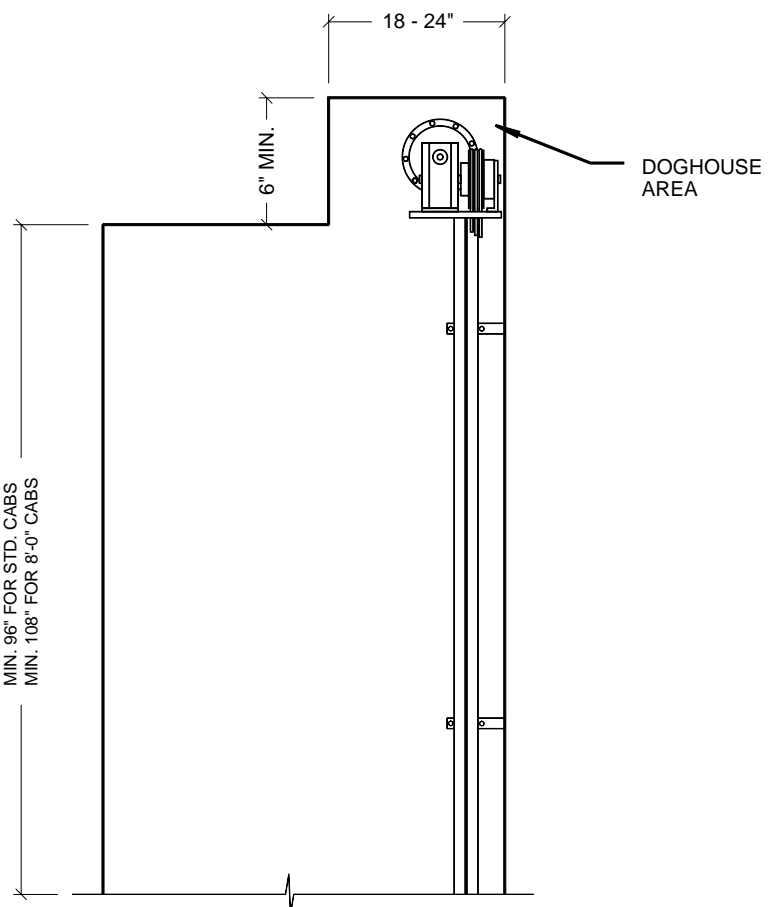
ELEVATION VIEW 'A'
