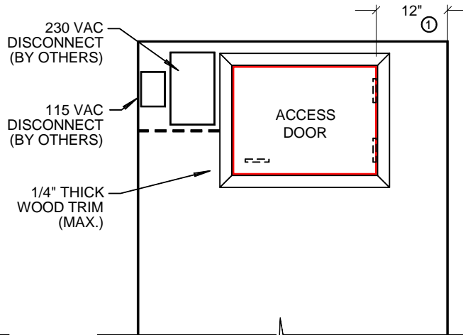
ELEVATION VIEW 'B'
