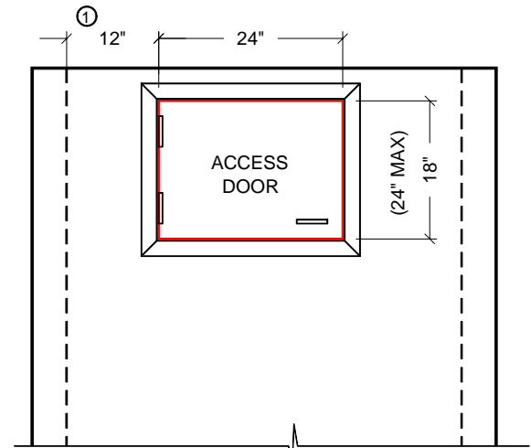
ELEVATION VIEW 'E'
