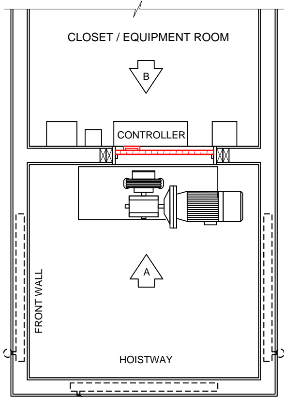
PLAN VIEW
