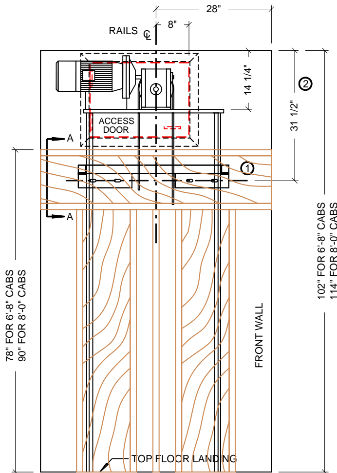
ELEVATION VIEW 'A'
