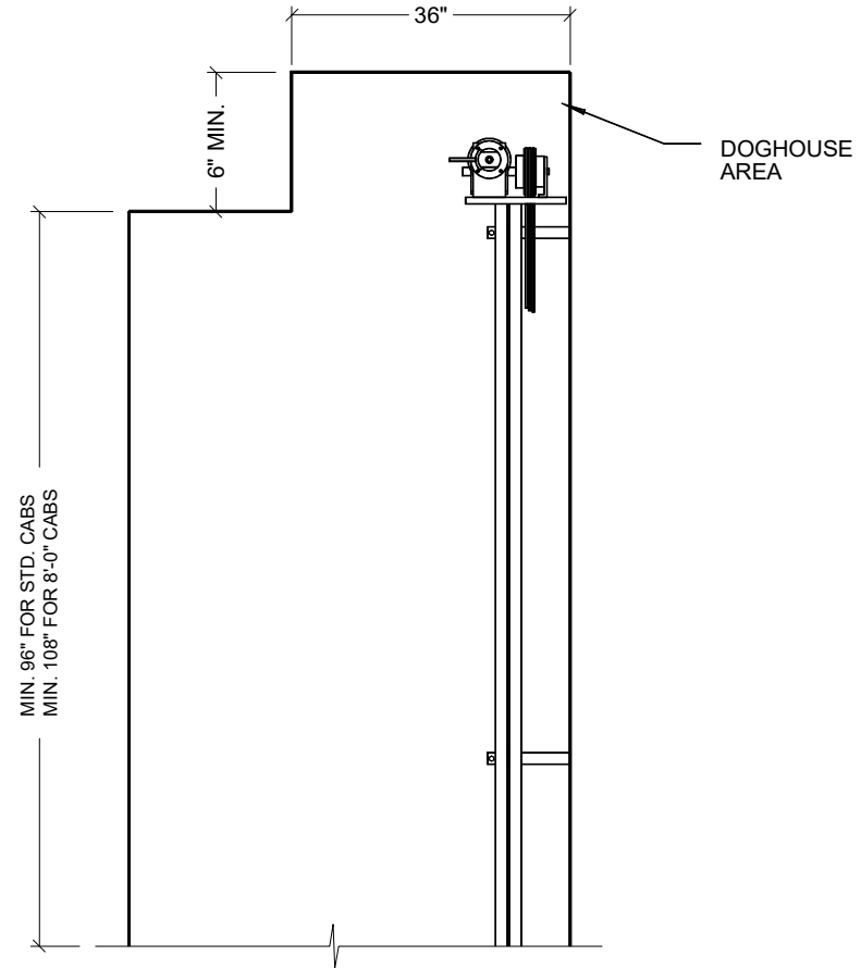
ELEVATION VIEW 'A'
