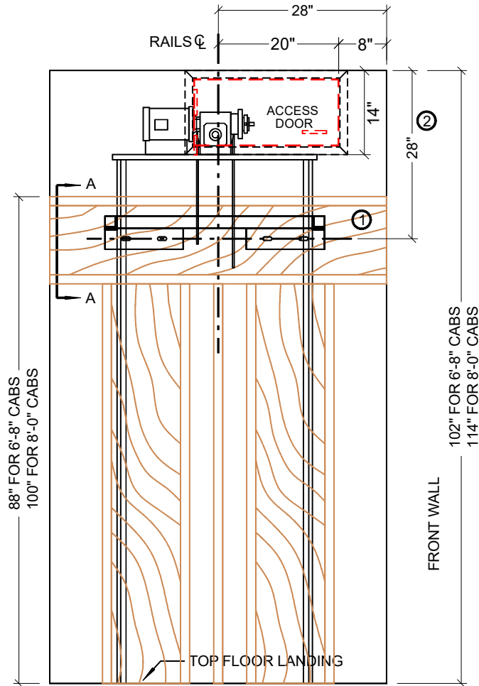
ELEVATION VIEW 'A'
